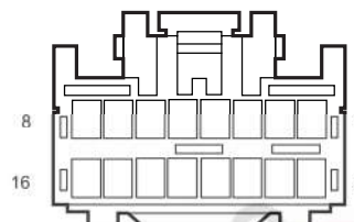
F26 Amplifier Assembly 2
