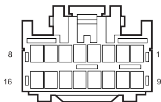
F26 Amplifier Assembly2
