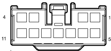
F02 Cabin Fuse Box G
