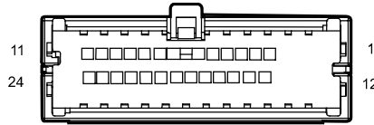
I4_MB Main W.H. Connector 4 Connecting Body W.H.
