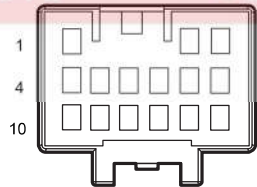
I_BRRD Body W.H. Connector Connecting RR Door W.H.
