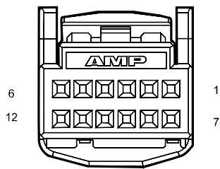
M40 Auto-release SW
