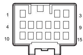
I_BRRD Body W.H. Connector Connecting RR Door W.H.
