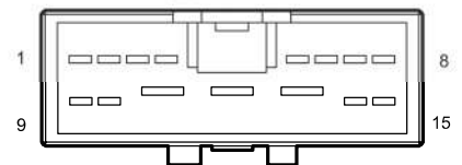
I2_BTBody W.H. Connector 2 Connecting Tailgate W.H.
