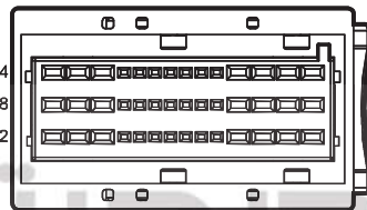
I1_EF Engine Harness to Body Harness I
