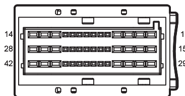
I1_EF Engine Harness to Body Harness 1
