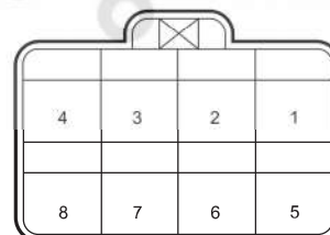
E06 FL Combination Lamp
