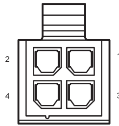
F47 Rear USB Connector
