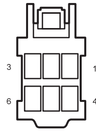
F29 Electrical Tailgate Controller 2
