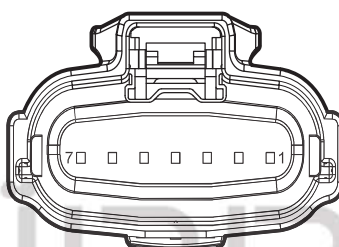
D18 Electrical Left Rear Door Lock
