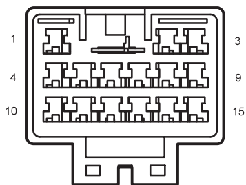
I3_FD Body Harness to Left Rear Door
