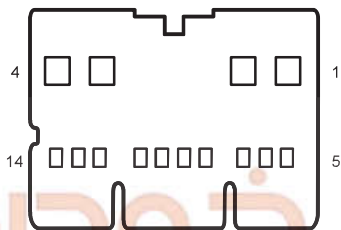
F30 Electrical Tailgate Controller 3
