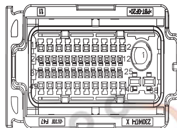
I1_DF Left Front Door to Body Harness
