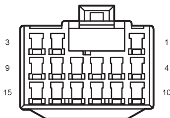
I4_DF Right Rear Door to Body Harness
