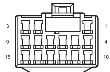
I3_DF Left Rear Door to Body Harness
