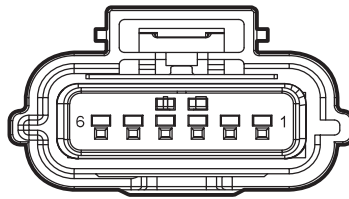
D28 Right Rear Door Lock
