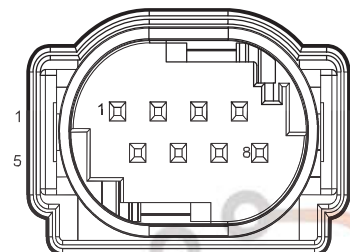
W04 Tailgate Closing Switch
