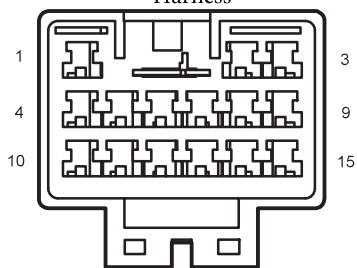
I3_FD Body Harness to Left Door Harness
