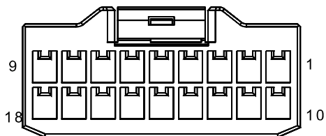
I2_TF Tailgate Transition Harness to Body Harness
