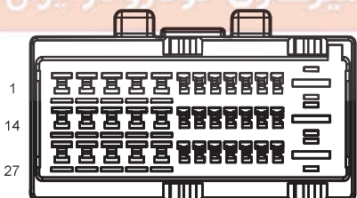
I1_FM Body Harness to Main Harness I
