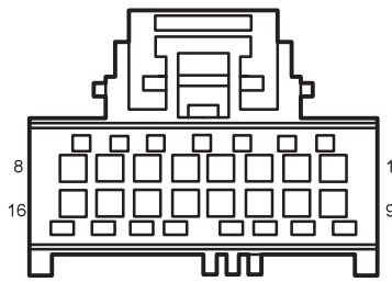
F28 Electrical Tailgate Controller 1
