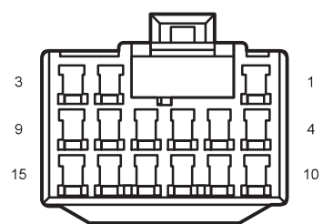
I3_DF Left Rear Door to Body Harness
