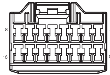
I2_TF Tailgate Transition Harness to Body Harness
