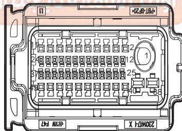
I2_DF Right Front Door to Body Harness
