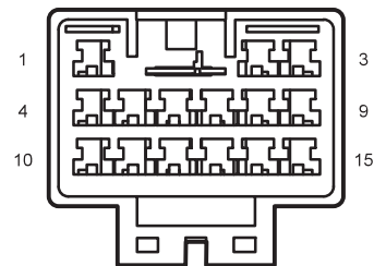
I4_FD Body Harness to Right Rear Door
