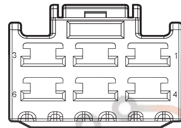
I2_EF Engine Harness to Body Harness 2
