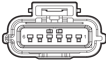
D16 Right Front Door Lock
