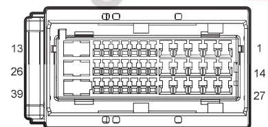
I1_MF Main Harness to Body Harness I
