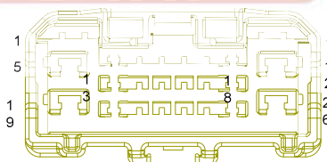
I1_FT Body Harness to Tailgate Transition Harness
