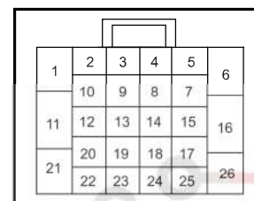
I1_BRPA Body W.H. Connector 1 Connecting Reversing Radar W.H.
