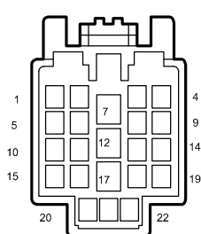
I1_BE Body W.H. Connector 1 Connecting Engine W.H.
