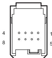
F08 Electronic Shifter Controller Connector 1
