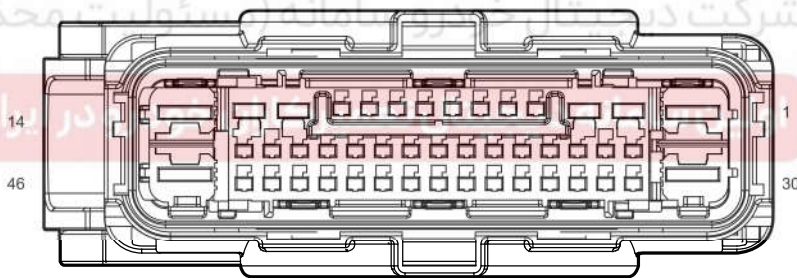
1.5T Engine EMS Connector
