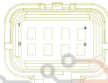
W11 Right Rear Inner Combination Light
