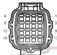
I1_FP Body Harness to Reverse Radar Harness I1_PReverse Radar Harness to Body Harness
