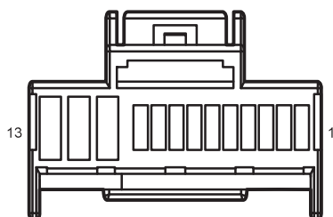
M06 Combination Switch-Light
