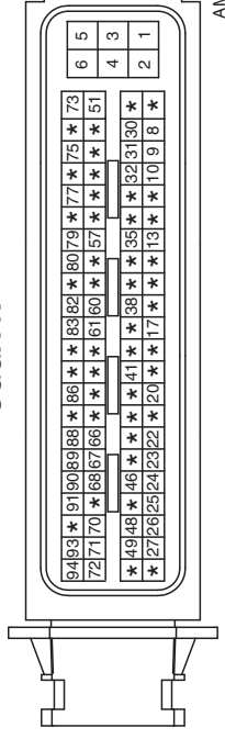
CGGA-K
