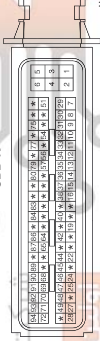
CDD-K
