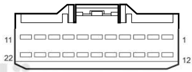
I1_RM Roof W.H. Connector 1 Connecting Main W.H.
