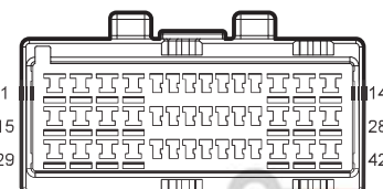
I1_FE Body Harness to Engine Harness 1
