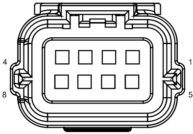
F14 Right rear combination lamp
