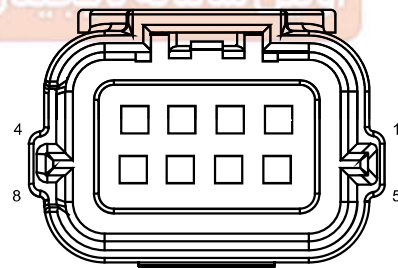
F19 Left rear combination lamp
