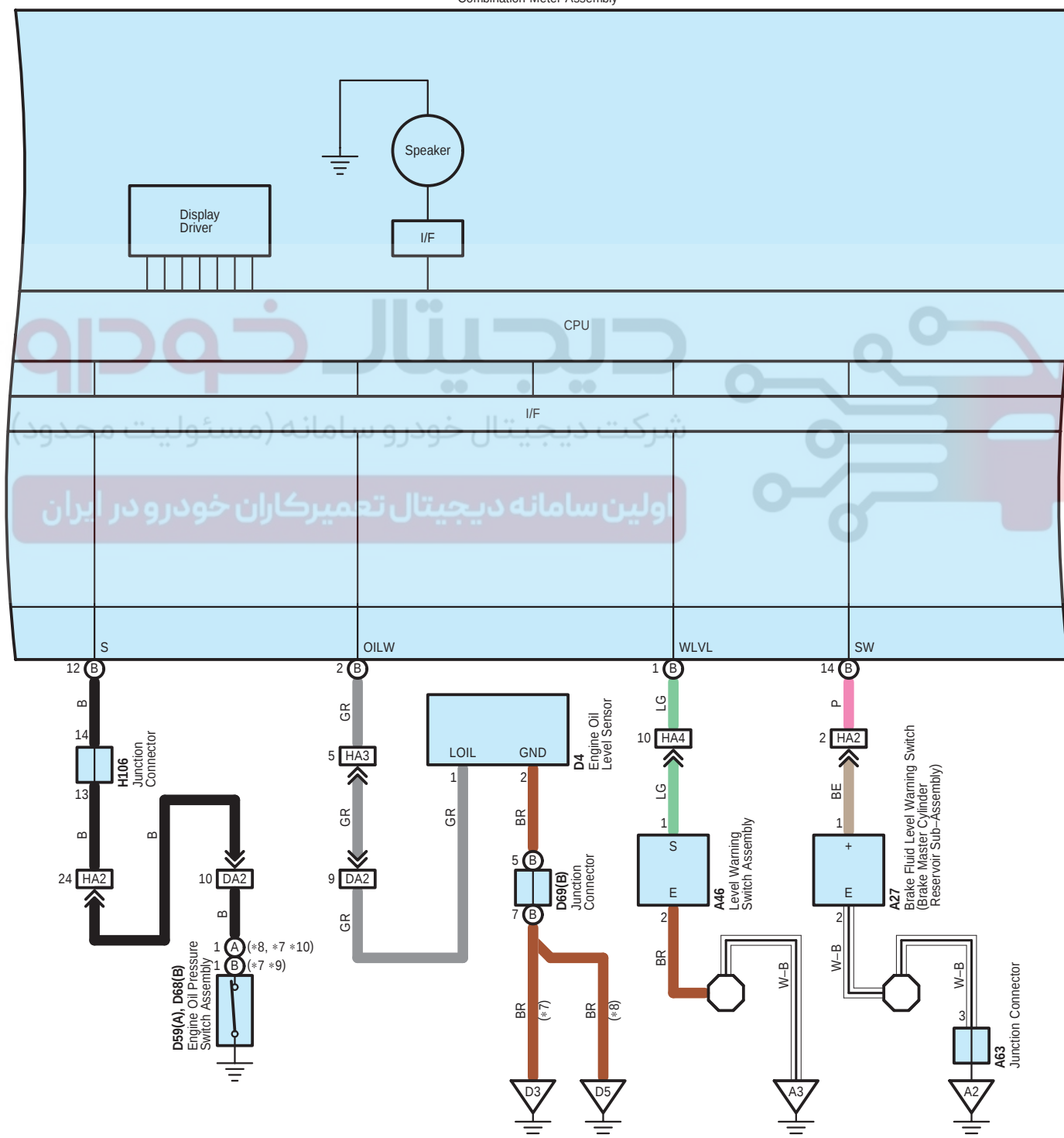
H13(A), H14(B) Combination Meter Assembly
