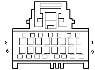
F52 Power Tailgate Controller
