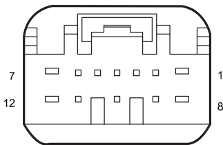
R12 Sunroof Motor
