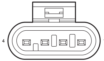
P07 Kick Sensor
