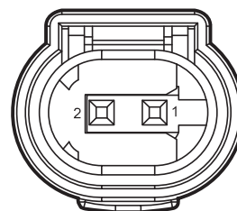
M19 PEPS Low Frequency Antenna 1
