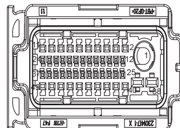
I1_DF Left Front Door Harness to Body Harness 1
