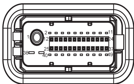
I2_FD Body Harness to Right Front Door Harness 1
