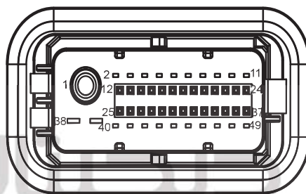
I1_FD Body Harness to Left Front Door Harness 1
