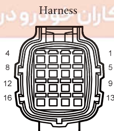
I1_PF Reverse Radar Harness to Body
