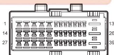
I2_FM Body Harness to Main
