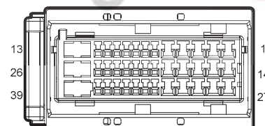
I2_MF Main Harness to Body
