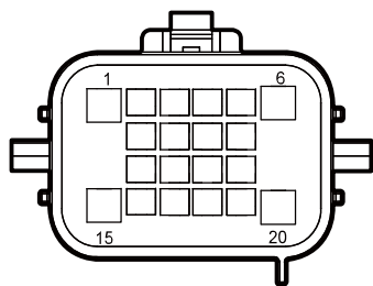
A24 To Vehicle Harness
