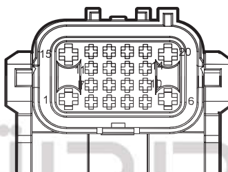
I3_EC Engine Harness to Control Harness -1.5T
