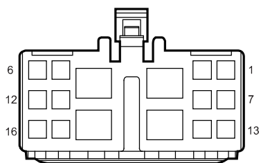
E41 Cabin Fuse Box A
