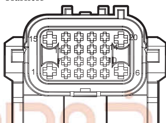
I3_EC Engine Harness to Control Harness
