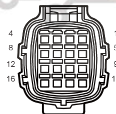
I1_PF Reverse Radar Harness to Body Harness
