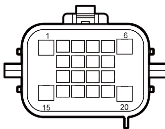
A24 To Vehicle Harness
