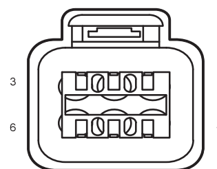
I1_BE Power Harness to Engine Harness
