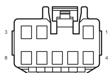
D33 Right Front Door Switch(Low Spec)
