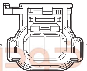
D34 Left Front Window Motor (Low Spec)
