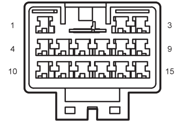
I4_FD Body Harness to Right Rear Door Harness
