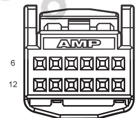
R11 Front Inner Roof Lamp
