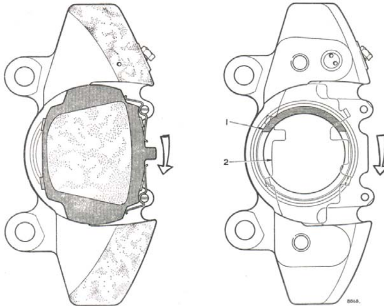
1. MACHINED STEP 2. ANTI-SQUEAK SHIM Fig. 3 Section through caliper showing correct location of the shim and anti-squeak step machined on outer end of piston which must always be positioned as shown
