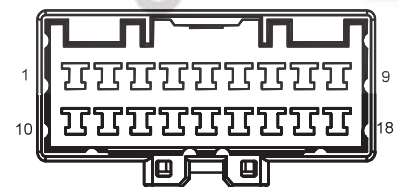
I1_RM Roof Harness to Main Harness 1
