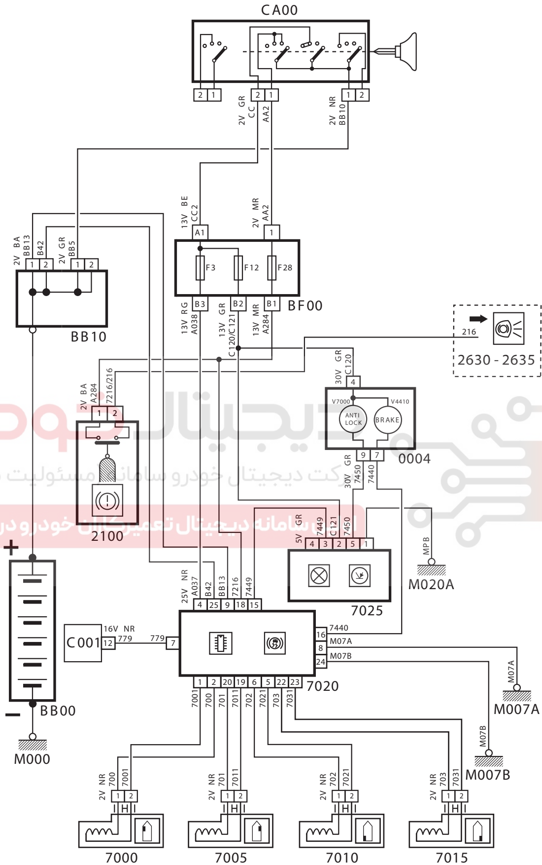
ANTILOCK BRAKE SYSTEM (ABS)
