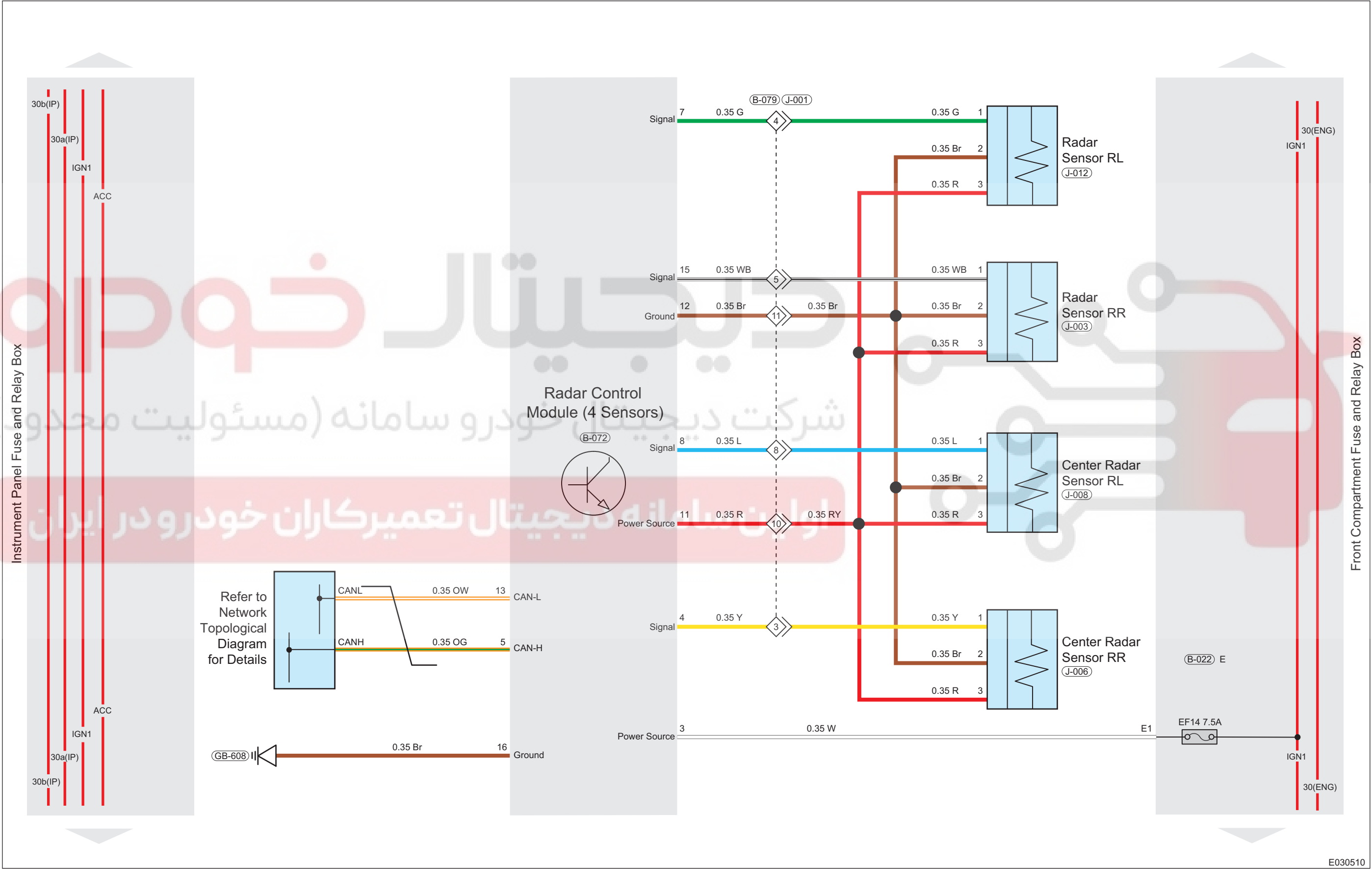
(16). Radar System (4 Sensors)
