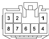
D33-1 Left rear door glass lift switch
