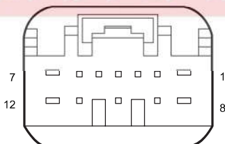
F36 Sunroof Motor(Top-line )
