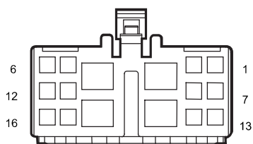
M05 Cabin Fuse Box M
