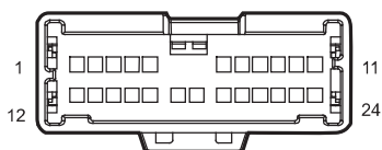
I2_MB Main W.H. Connector 2 Connecting Body W.H.
