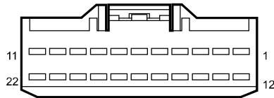
I1_RM Roof W.H. Connector 1 Connecting Main W.H.
