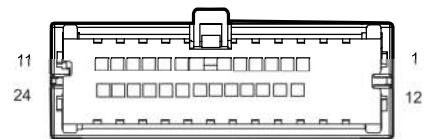
I4_MB Main W.H. Connector 4 Connecting Body W.H.
