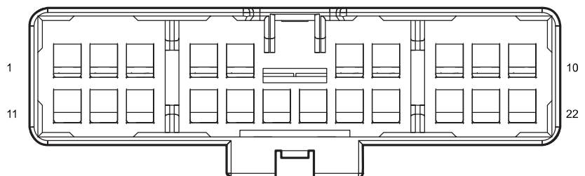
I1_BT Body W.H. Connector 1 Connecting Tailgate W.H.
