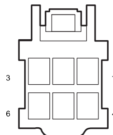
F53 Power Tailgate Controller 2
