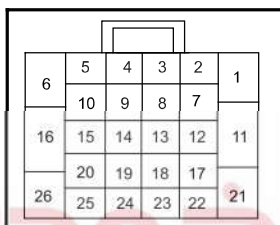
I1_RPAB Reversing Radar W.H. Connector 1 Connecting Body W.H.
