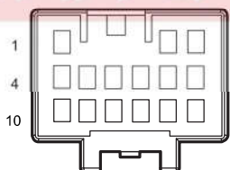
I_BRRD Body W.H. Connector Connecting RR Door W.H. F50 Fuel Tank Cap Actuator
