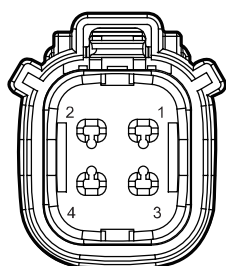
T09 Tailgate Outer SW
