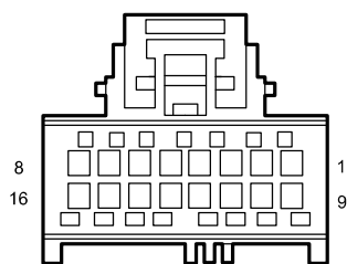
F52 Power Tailgate Controller
