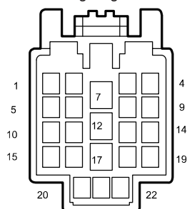
I1_BE Body W.H. Connector 1 Connecting Engine W.H.
